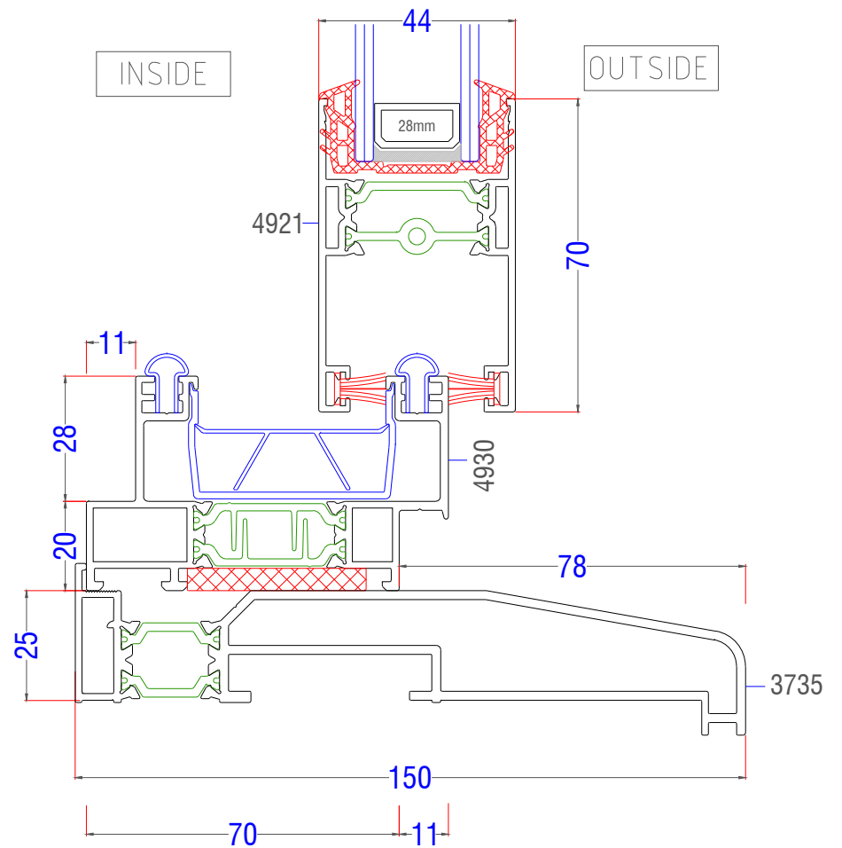
150mm Cill
