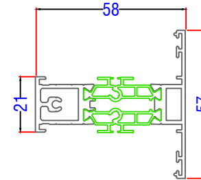
U44045 - Mullion/Transom
