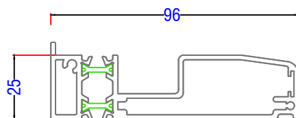
AL UK AW570 - 95mm Stub Cill
