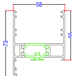
AL UK AW608 - Outer Frame
