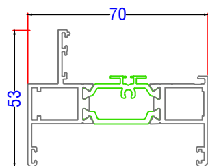
ALU UK AW622 - Outer Frame
