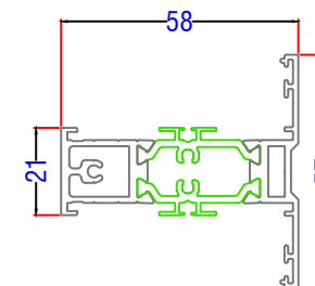
AL UK AW631 - Mullion/Transom
