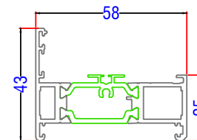
AL UK AW604 - Outer Frame
