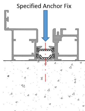
Typical outer frame installation
