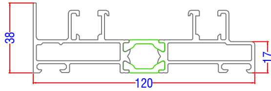
148040 - Dual Track Outer frame
