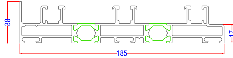
148100 - Triple track Outer Frame
