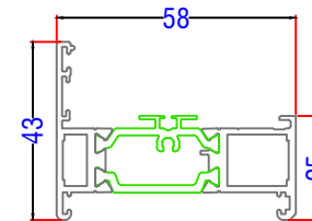
AL UK AW604 - Outer Frame
