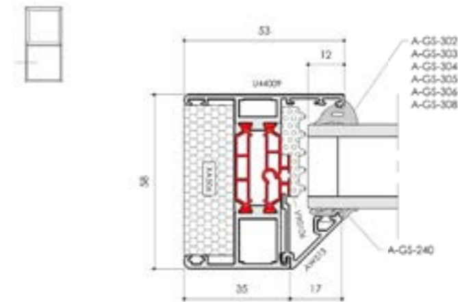
Fixed Jamb Detail
